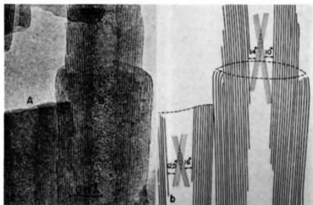
Fig. 9. Conical fibril in which the 7.3 Å lattice fringes on opposite sides are not parallel to each other (synthetic sample). The conically tapered angles are 3° (A) and 5.5° (B). (b) is a drawing of the fringe systems.
